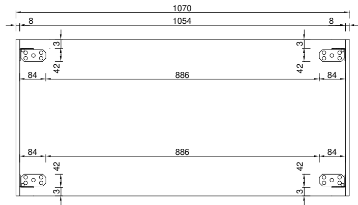
c1, c2, c3 covers Front view
