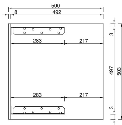
c1, c2, c3 covers Side view
