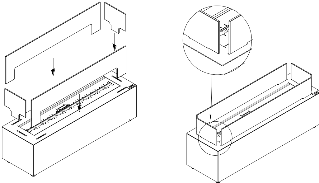
Fig. 4 – Glass installation
