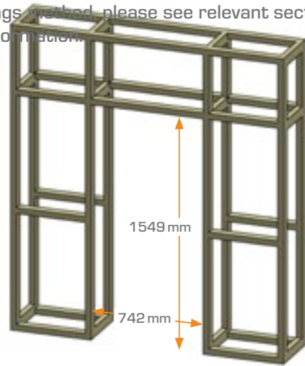
OPEN DIMENSIONS FOR KNIGHTWOOD STUDWALL INSTALLATION
