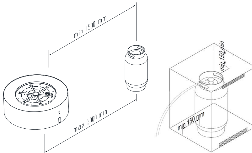
Fig. 4 – Gas cylinder distance
