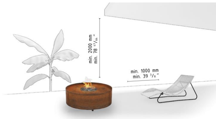
Fig. 1: Minimum distance to flammable materials
